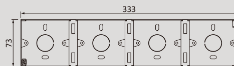
M1474 4 Gang Metal Wall Box
