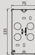
M1047D 2 Gang Metal Wall Box
