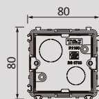
R1150 1 Gang Plastic Wall Box
