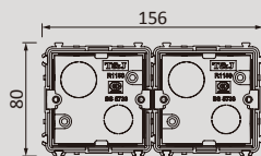
R1150 2 x 1 Gang Plastic Coupling Wall Box
