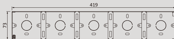
M1475 5 Gang Metal Wall Box
