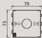
M1247 1 Gang Metal Wall Box
