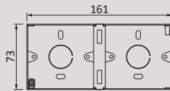
M1472 2 Gang Metal Wall Box
