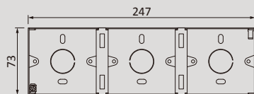
M1473 3 Gang Metal Wall Box
