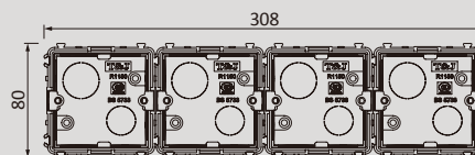
R1150 4x 1 Gang Plastic Coupling Wall Box
