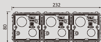
R1150 3x 1 Gang Plastic Coupling Wall Box
